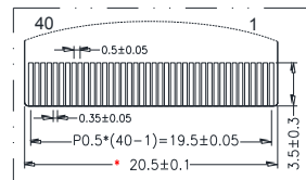
DETAIL A(2.5:1)
